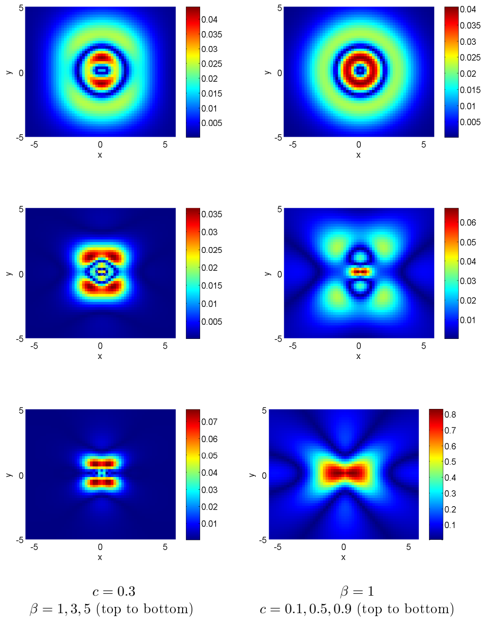
Fig. 5. Difference between the numerical solution v and best fit formulae v^* from [5]
