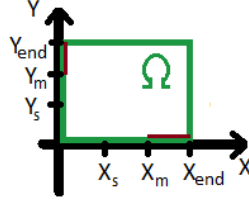
Fig. 1. Stop Criteria Intervals
