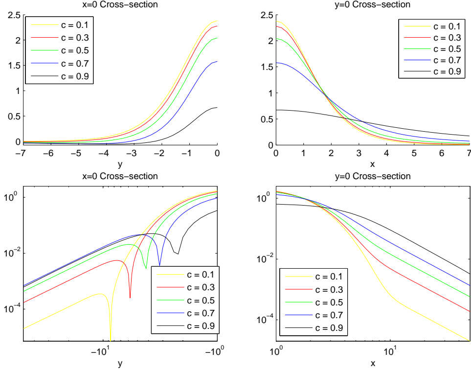
Fig. 4. Cross-sections of the numerical solution for \beta = 1 and several c
