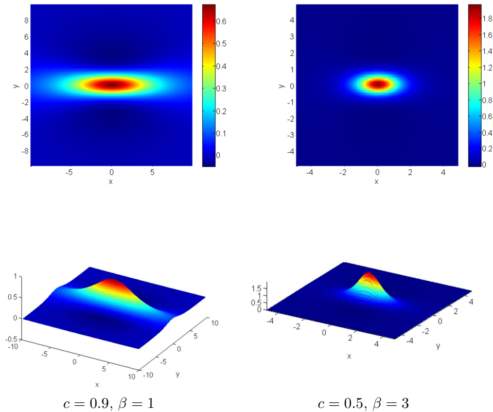
Fig. 3. 2D and 3D profiles of the numerical solution u to (8) and (9)
