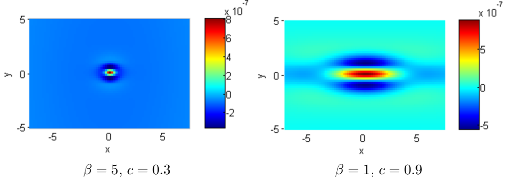
Fig. 2. Residual at the last step of iteration process (11)
