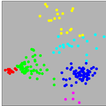
Fig. 8. An MDS plot of 6 clusters produced by WPGMA. Note that the good separation of the clusters is often spoiled by unclear margins
